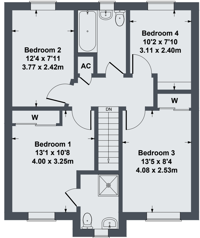
FIRST FLOOR
